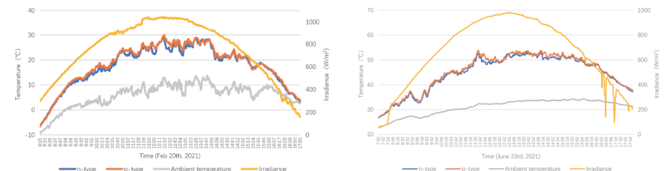
Figure 5 : Operational temperature comparison of n-type and p-type PERC modules
